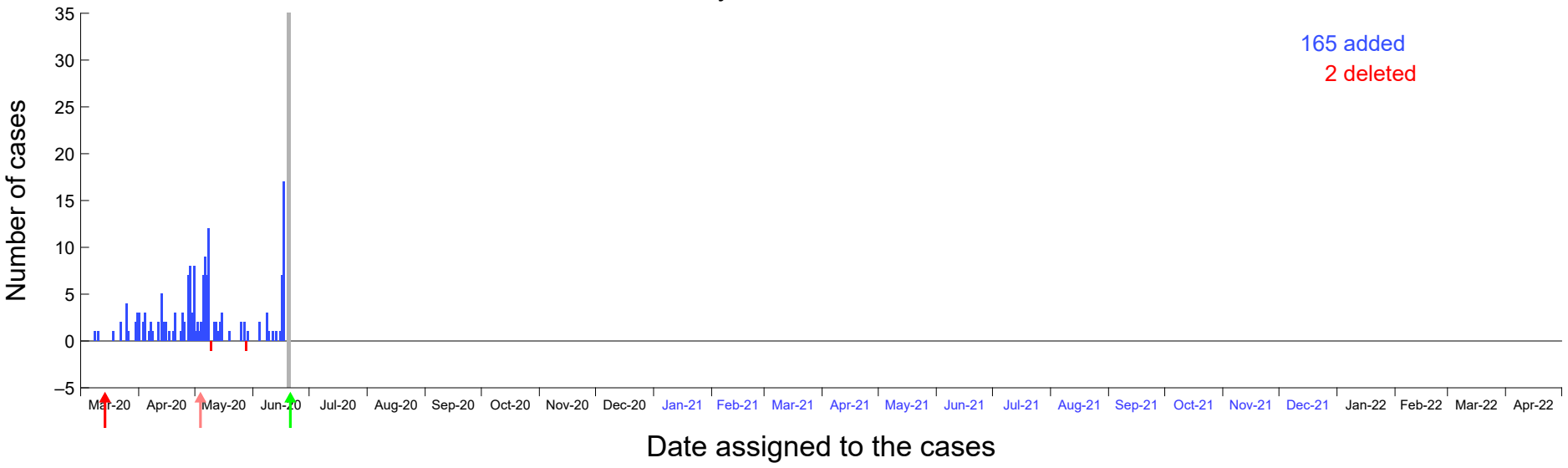
Distribution of delayed notifications on Jun 19th, 2020
