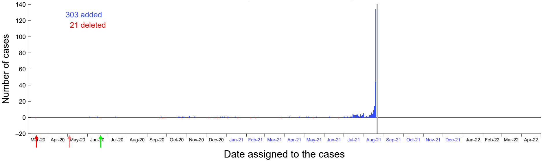
Distribution of delayed notifications on Aug 21st, 2021
